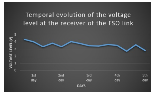
Fig. 3. Temporal behavior of the DC voltage level.
