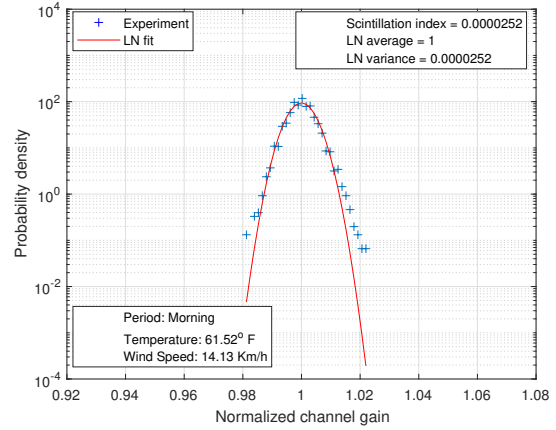
Fig. 7. Histogram of normalized channel gain and the LN density adjusted for a morning period and clear sky climatic conditions. Expected value of h , E[h] = 3.78 V.
