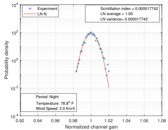
Fig. 8. Histogram of normalized channel gain and the LN density adjusted for a night period and clear sky climatic conditions. Expected value of h , E[h] = 4.4 V.
