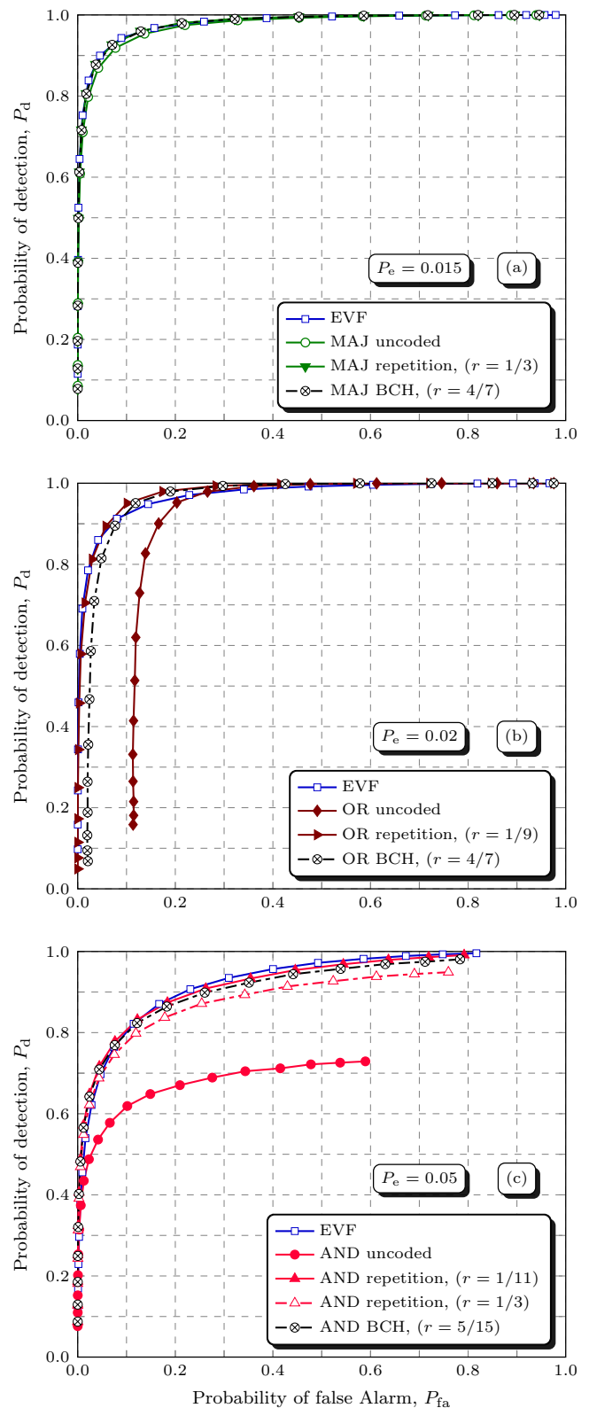
Fig. 7: ROCs for ED with channel coding for (a) EVF and DF MAJ, (b) OR and (c) AND.
