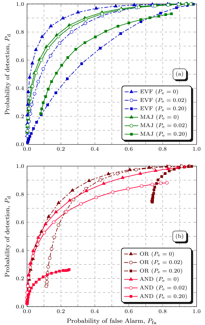
Fig. 6: ROCs for MMED without channel coding and different P_e values for (a) EVF and DF MAJ, (b) OR and AND.
