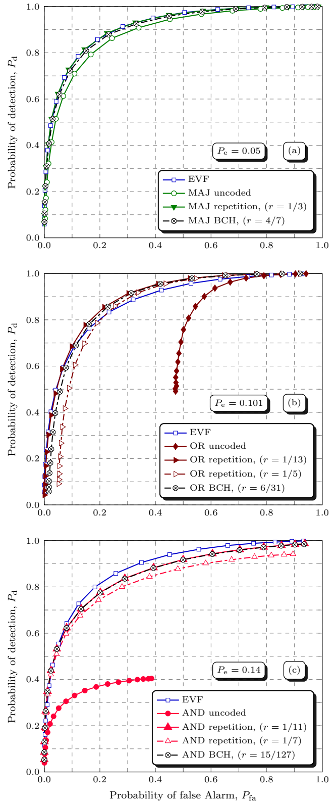
Fig. 9: ROCs for GLRT with channel coding for (a) EVF and DF MAJ, (b) OR and (c) AND.
