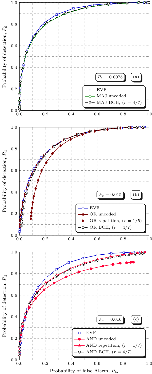
Fig. 10: ROCs for MMED with channel coding for (a) EVF and DF MAJ, (b) OR and (c) AND.
