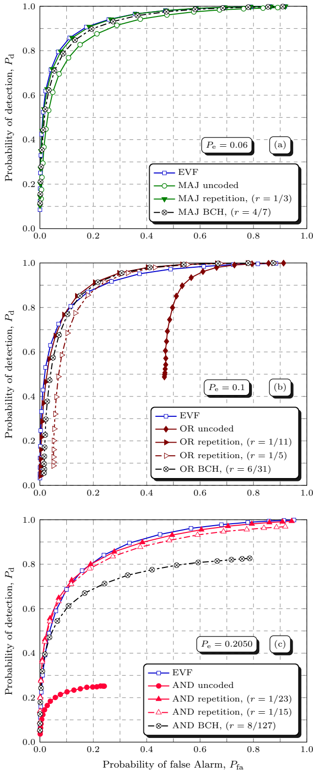
Fig. 8: ROCs for MED with channel coding for (a) EVF and DF MAJ, (b) OR and (c) AND.
