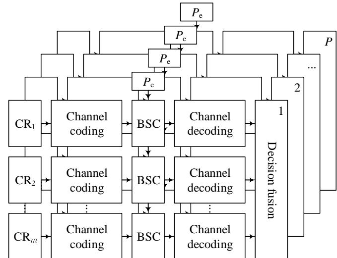
Fig. 2: Decision fusion (DF) diagram for detecting OFDMA subchannels.
