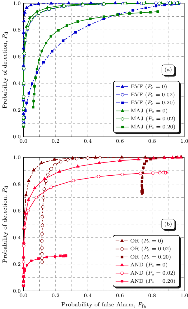
Fig. 3: ROCs for ED without channel coding and different P_e values for (a) EVF and DF MAJ, (b) OR and AND.
