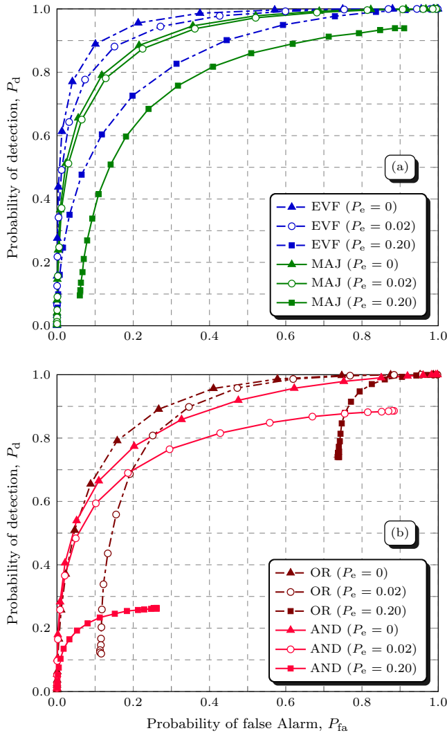
Fig. 5: ROCs for GLRT without channel coding and different P_e values for (a) EVF and DF MAJ, (b) OR and AND.
