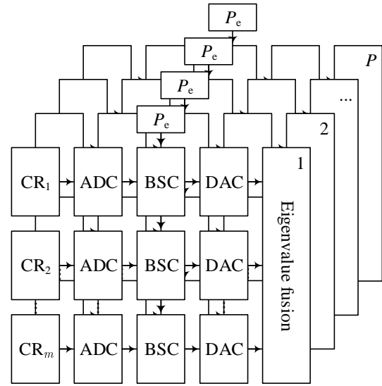
Fig. 1: Eigenvalue fusion (EVF) diagram for detecting OFDMA subchannels.
