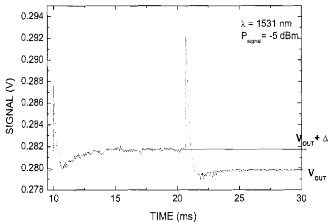
Figure 3. Experimental signal recorded over one polarization switching period during the determination of the PDG.
