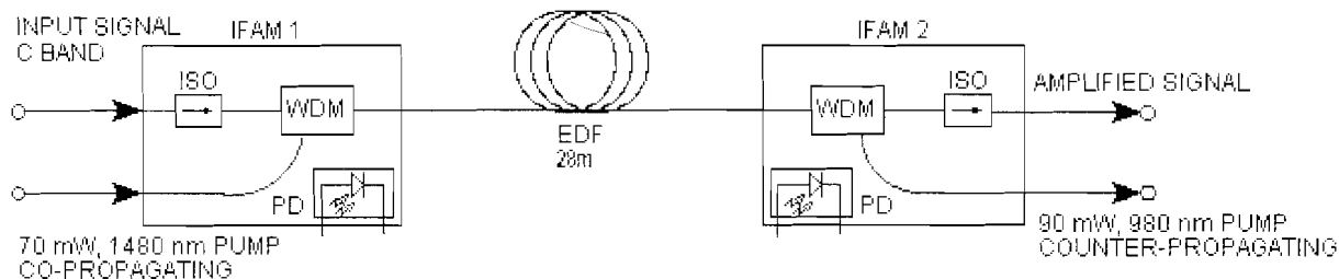
Figure 1. Schematics of the used EDFA, after [19].
